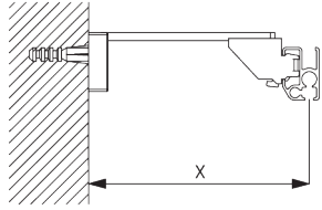
Smart Fix squadro SG 11210 - SG 11215 e supporto SG 3603: Necessaria vite SG 10492 (M4x8).
