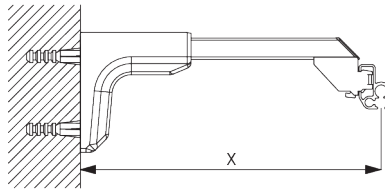
Smart Fix universale SG 11154 - SG 11156 e supporto SG 3603: Necessaria vite SG 10277 (M4x12).
