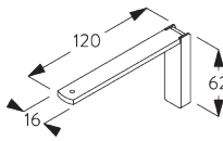
SG 11203 Smart Fix 120 mm
