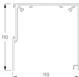
SG 11533 Astuccio 110 mm
