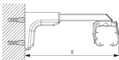
Smart Fix universale SG 11154 - SG 11156 e supporto SG 2302: Necessaria vite SG 10492 (M4x8).
